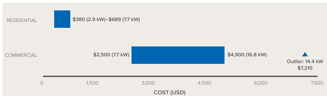
Range of Level 2 charger costs.
